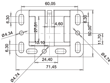
4600-BRKTSO Screw On Rear Adjustable Socket
