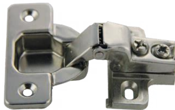
Short Arm Face Frame Hinge = 1/2" Overlay
